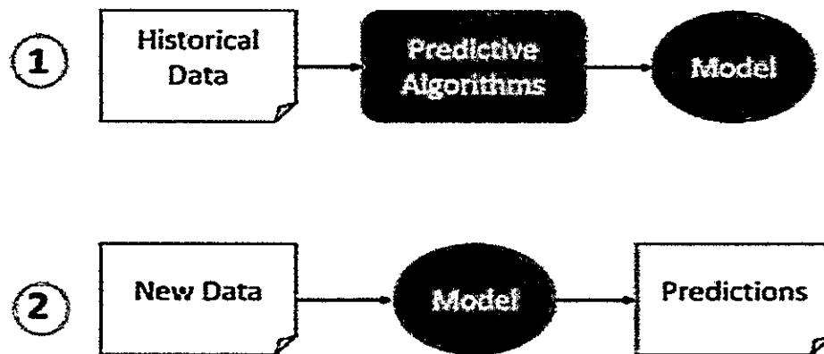
Fig. 3. Predictive model.
